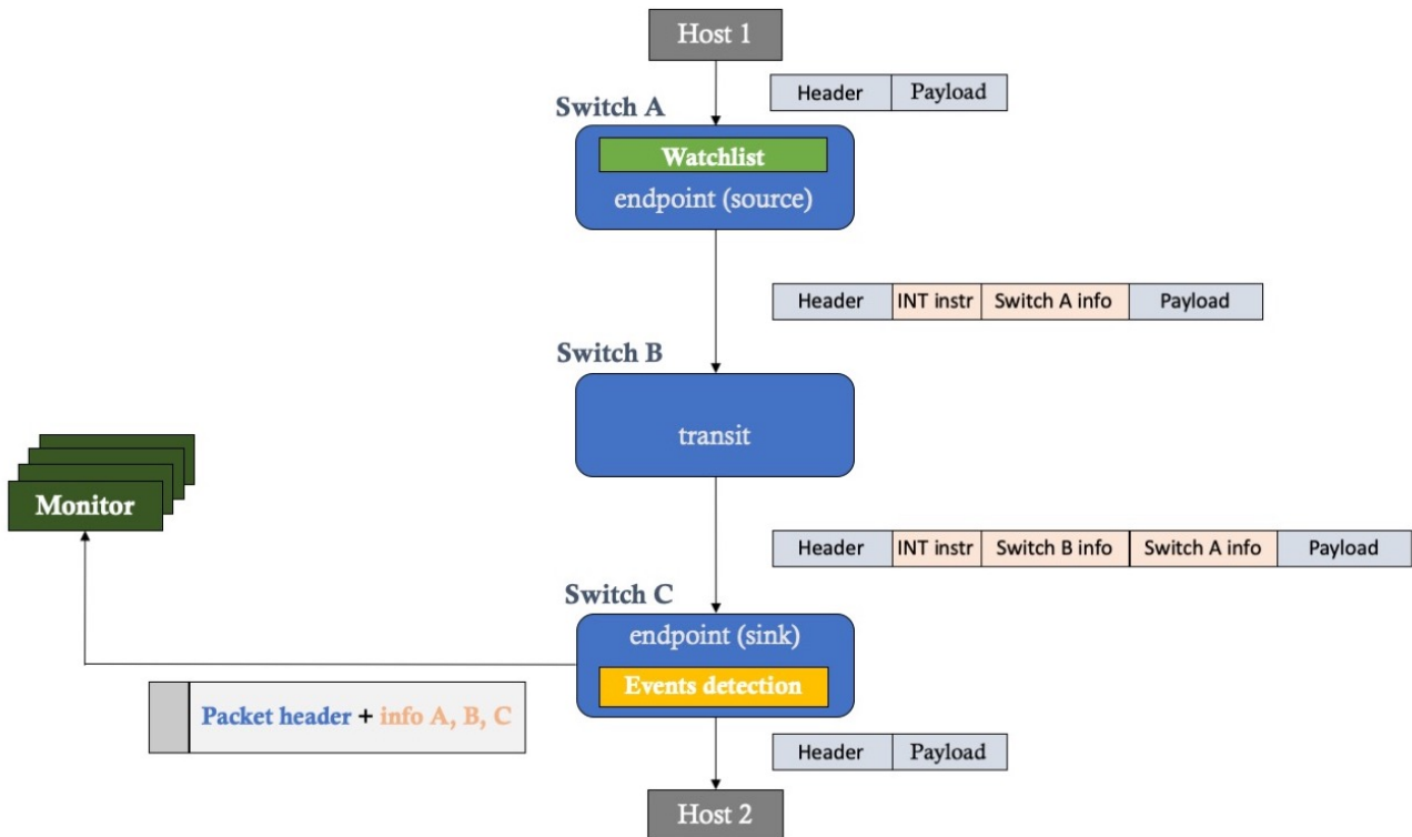
Figure 3. INT-MD mode - Telemetry Architecture with stacked reports generated by sink nodes
